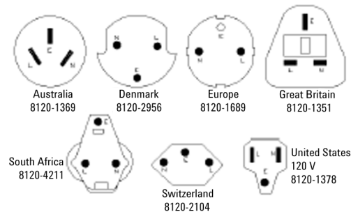
Figure 9 Line Power Cables - Plug Identification
