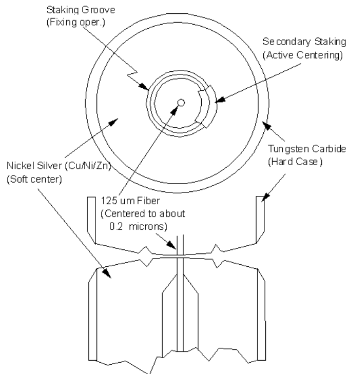
Figure 4 Cross-section of the Diamond HMS-10 connector.
