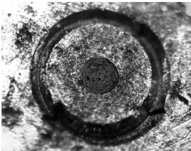
Figure 6 Dirty fiber end and ferrule from poor cleaning.
