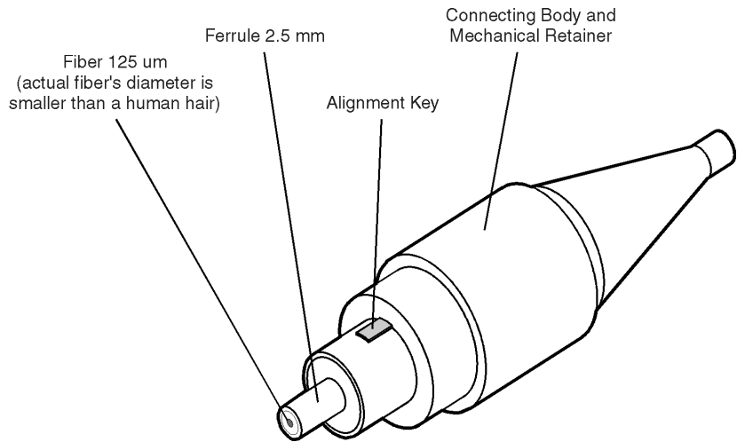
Figure 2 Basic components of a connector.
