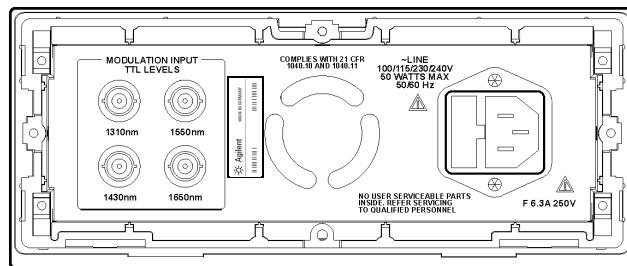
Figure 1 Rear view of instrument
